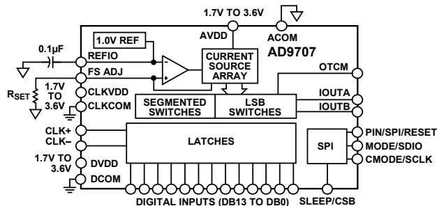
Figure 1. AD9707
